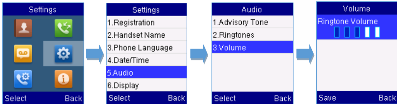
Figure 24: Ringer Volume
