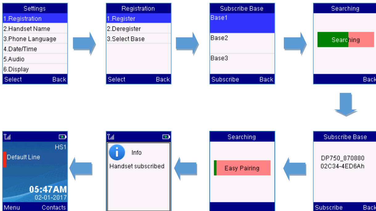
Figure 10: Registration process
